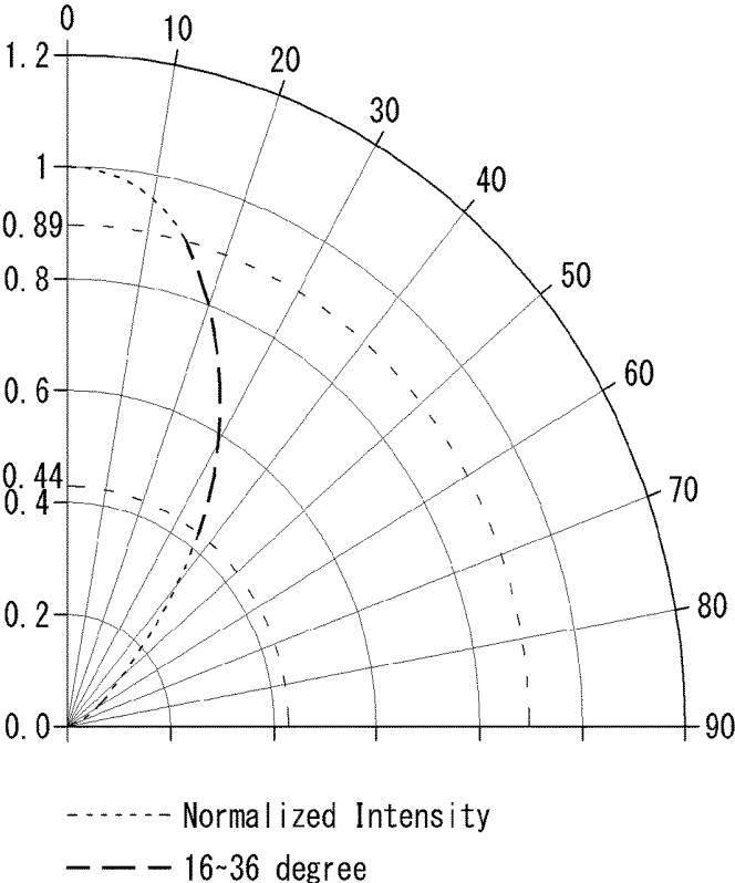
[Brightness variation with viewing angle of microcavity OLED device]
